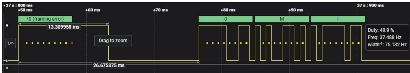
Figure 9. Oscillogram
