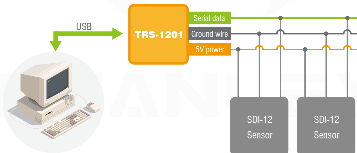
Figure 2. Principle diagram
