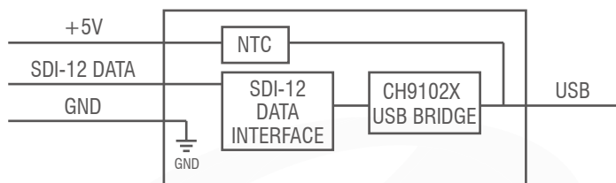
Figure 1. TRS-1201 block diagram
